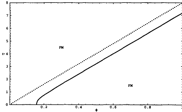
FIG. 2. Phase diagram for Ising dipoles. PM indicates paramagnet and FM indicates ferromagnet. The solid line is from generalized mean-field theory. The dotted line is from conventional mean-field theory.
