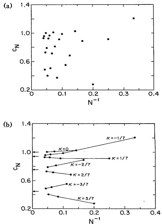
FIG. 1. (a) Numerical data for the FSS amplitudes of the free-fermion model for the domain-wall density d = \frac{1}{2} on an infinite cylinder of width N with periodic boundary conditions. c_N is proportional to the FSS amplitudes; c_N = (6/\pi\zeta)N^2(f_\infty - f_N) , where \zeta is the anisotropy factor. f_N is the exactly known ground-state energy for finite systems (Refs. 7 and 10) and f_\infty is the bulk term. (b) Classification of numerical data for different values of mismatch parameter \kappa . Arrows indicate the exact values of the conformal charge c_\infty obtained from Eq. (6). Lines between data points are only guides to the eye.
