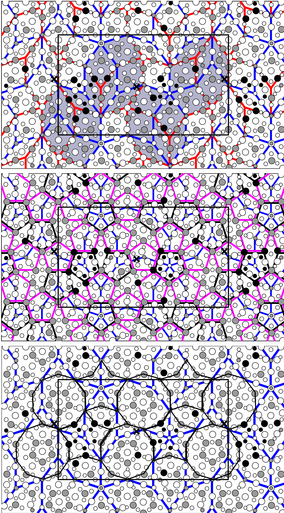
FIG. 1: Optimal realization of the W-phase. We show only a single 4 \text{ \AA} bilayer. The other is obtained by a translation of (a/2, 0, c/2) . (top) red and blue HBS tilings together outline binary rhombus tiling. Shaded regions are “octagons” that flip in the adjacent bilayer. (middle) PB clusters in violet centered on shared vertices of blue and red tilings. Black pentagons are alternate vertex type of blue tiling. (bottom) 13 \text{ \AA} decagonal clusters of Co-rich decagonal quasicrystal model.
